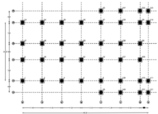
Figure 3. Layout of isolator joints in the FPS model.
