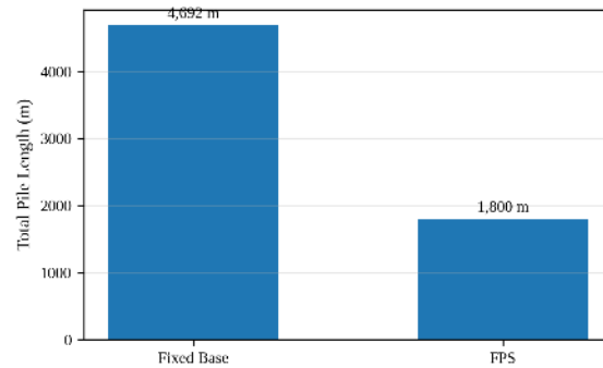
Figure 8. Total length comparison of 60 cm spun piles.
